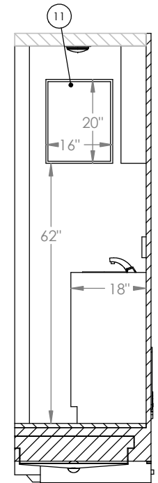
SECTION M-M
