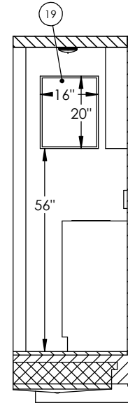
SECTION M-M
