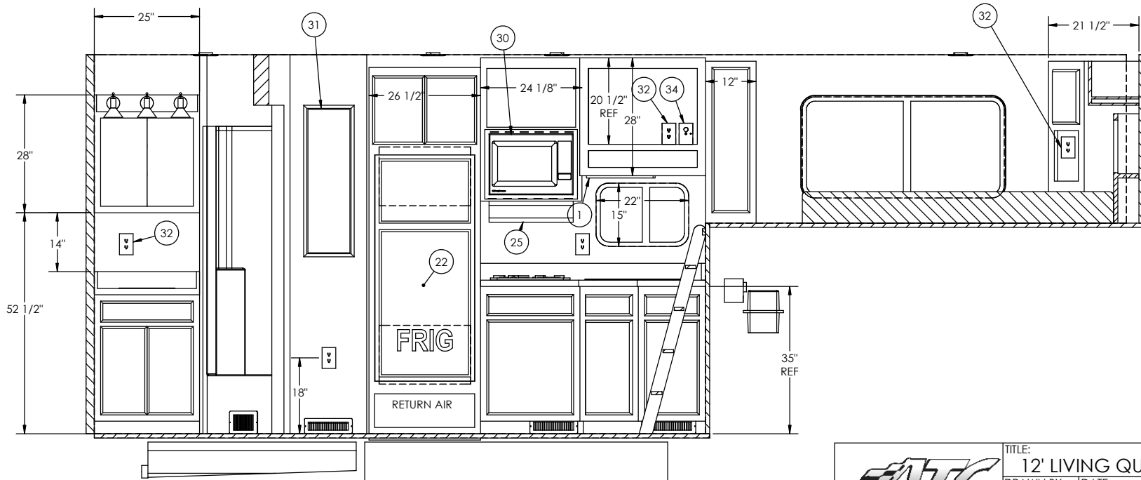
ROADSIDE INTERIOR SECTION B-B
