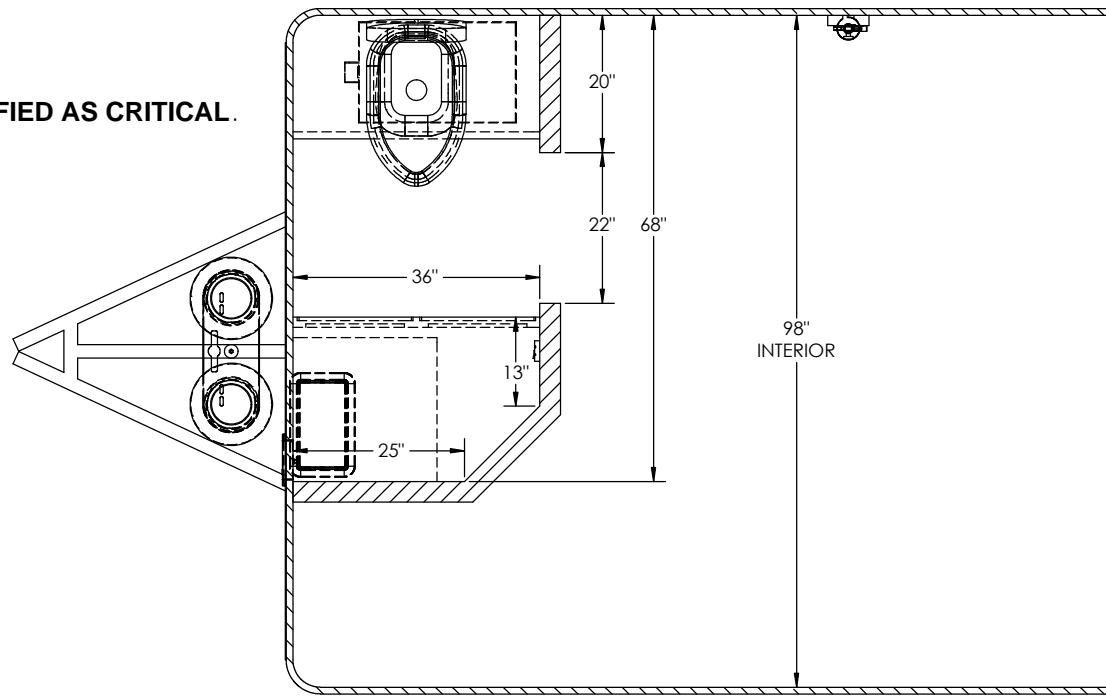
SECTION E-E
