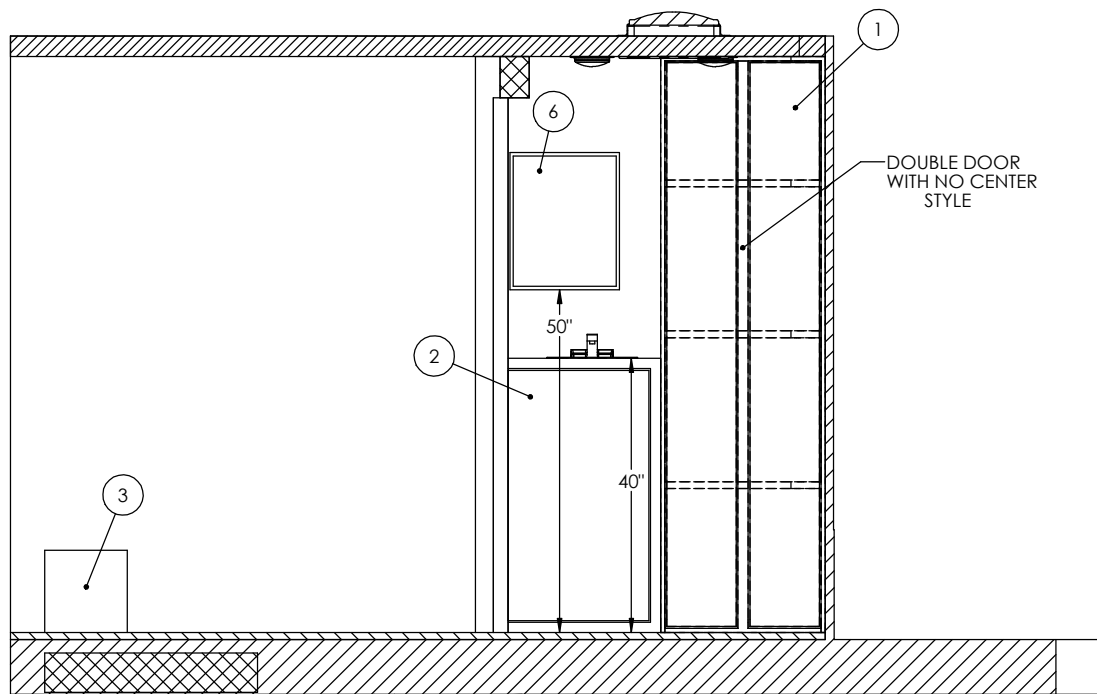
INTERIOR ROAD SIDE SECTION B-B
