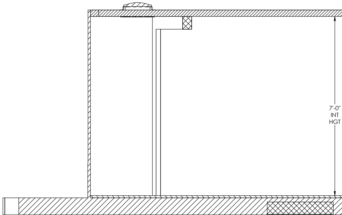
INTERIOR CURB SIDE SECTION A-A
