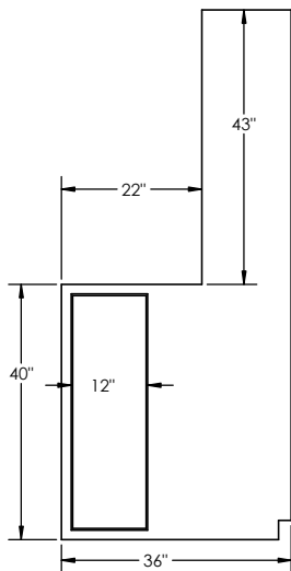
LAV BASE/ LINEN CLOSET FRONT VIEW
