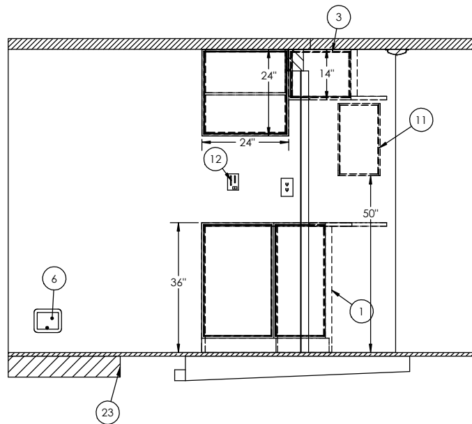
ROADSIDE INTERIOR SECTION B-B
