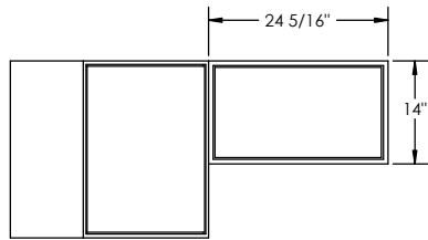
FRONT VIEW B
