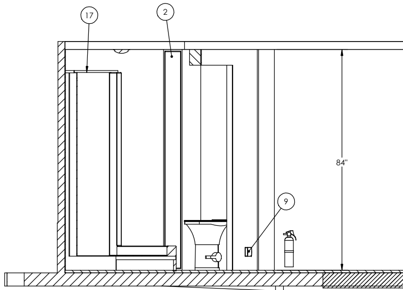
CURBSIDE INTERIOR SECTION A-A
