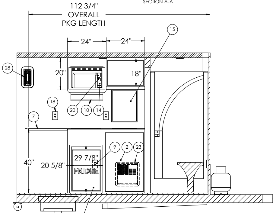
ROADSIDE INTERIOR SECTION B-B
