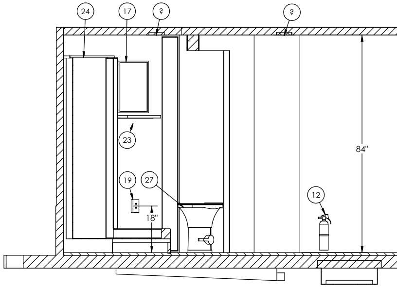
CURBSIDE INTERIOR SECTION A-A
