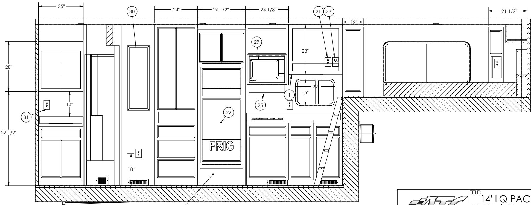
ROAD SIDE INTERIOR SECTION B-B
