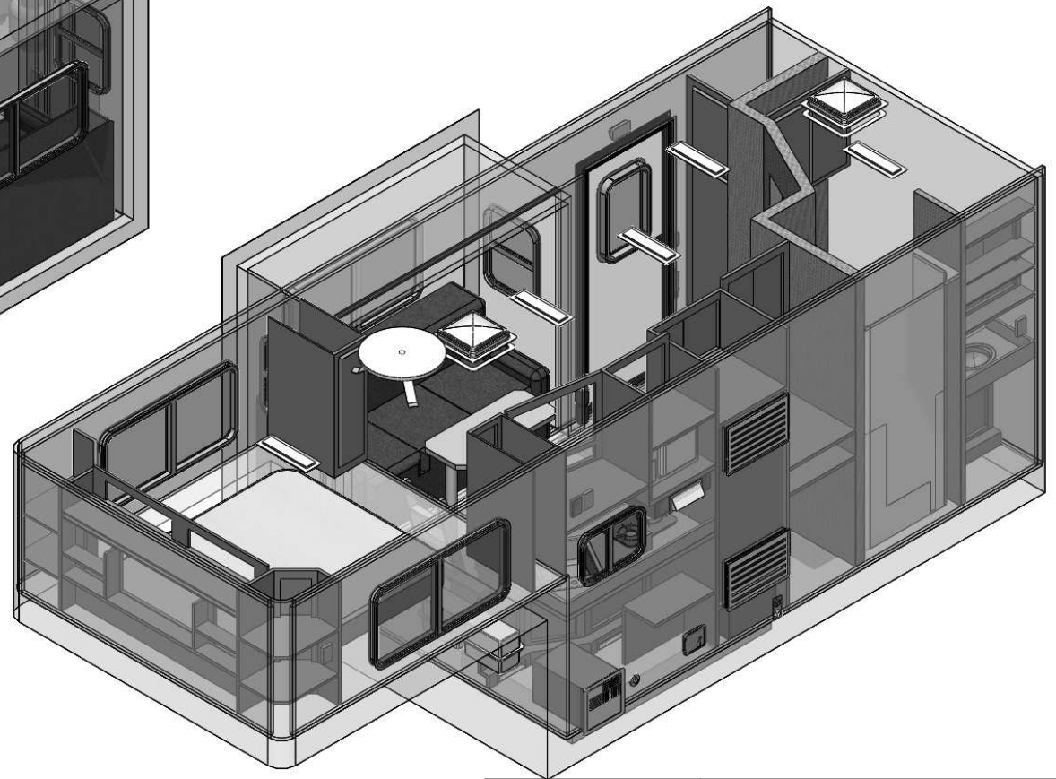
ROAD SIDE VIEW
