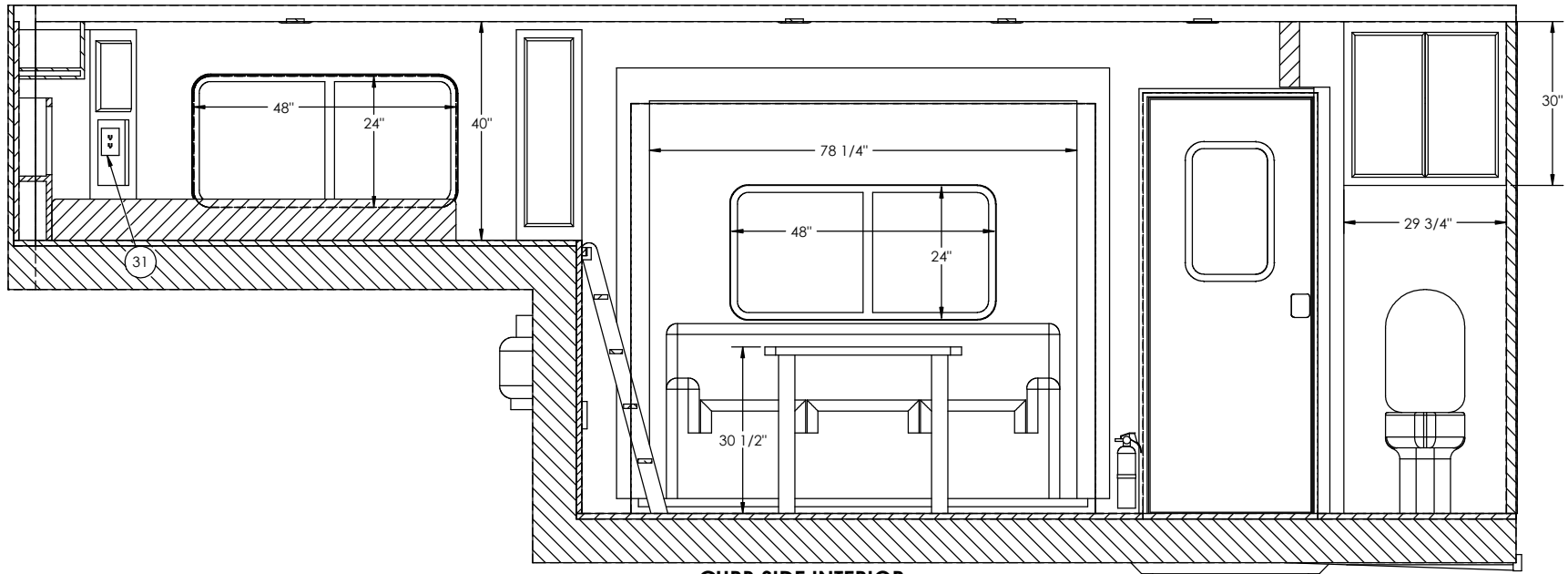
CURB SIDE INTERIOR SECTION A-A
