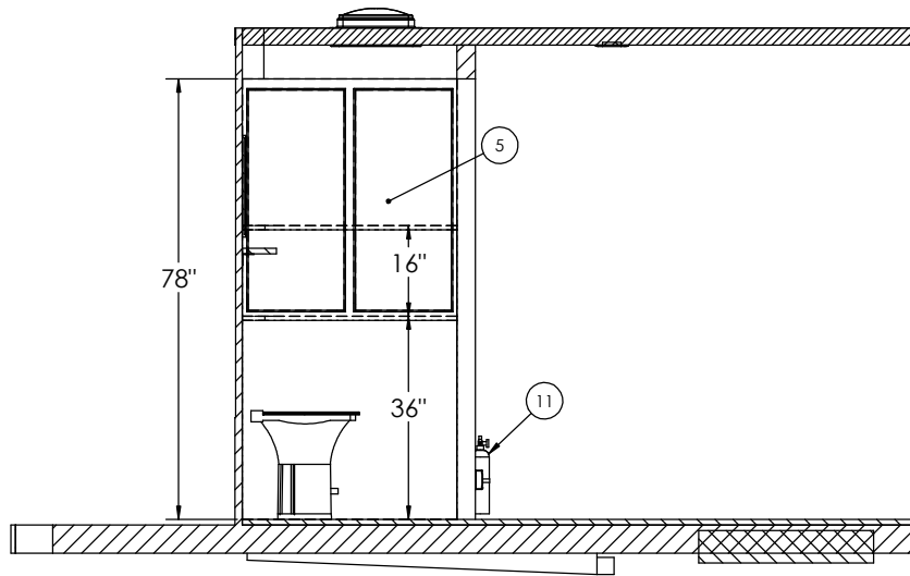
CURBSIDE INTERIOR SECTION A-A
