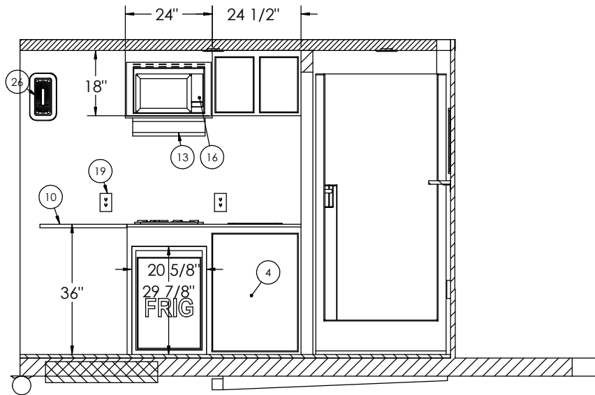
ROADSIDE INTERIOR SECTION B-B
